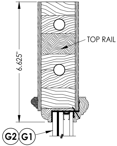
3 2 VERTICAL CROSS SECTION
