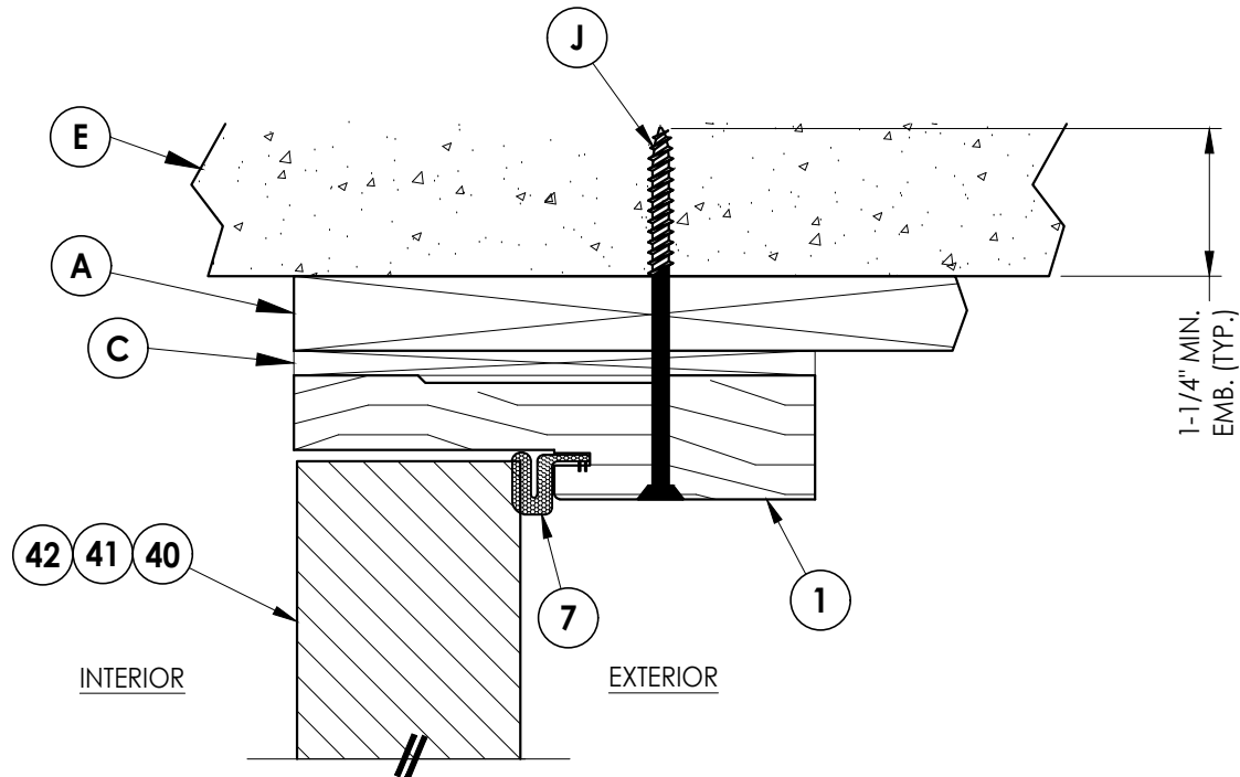
3 8 VERTICAL CROSS SECTION Shown w/ 1X sub-buck Inswing shown (Outswing similar)
